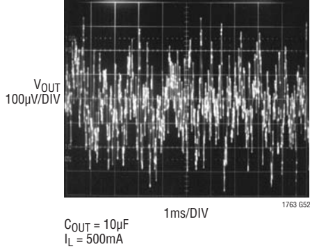
LT1763-5 10Hz to 100kHz Output Noise C_{BYP} = 0
