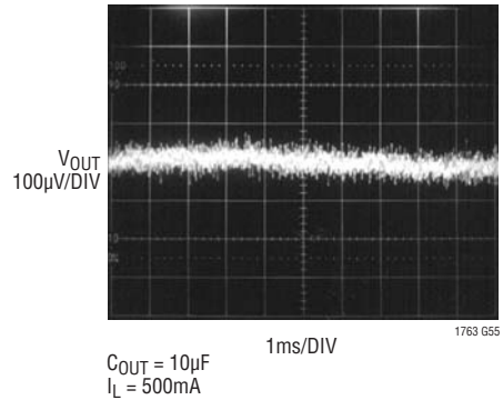
LT1763-5 10Hz to 100kHz Output Noise C_{BYP} = 0.01 \mu F
