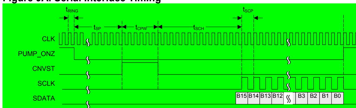
Figure 9A. Serial Interface Timing
