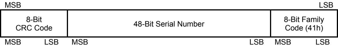
Figure 5. 64-Bit Lasered ROM
