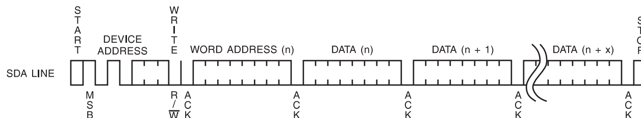
Figure 8-3. Page Write
